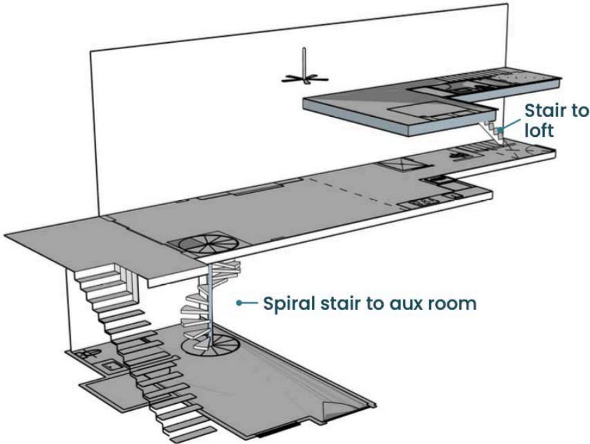
Exploded view of the three levels
